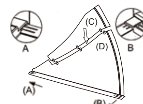
2. Carefully assemble the safety shield (C) on the safety shield (D). Insert the Safety Shield into the upper cap (A) and lower cap (B).
